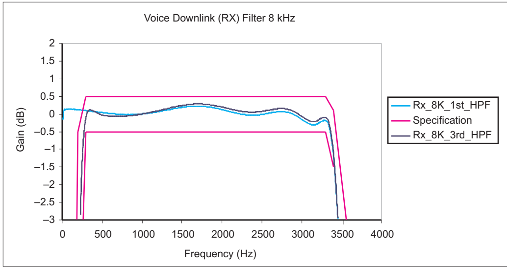
Figure 6-17. Voice Downlink Frequency Response With F_S = 8 kHz
