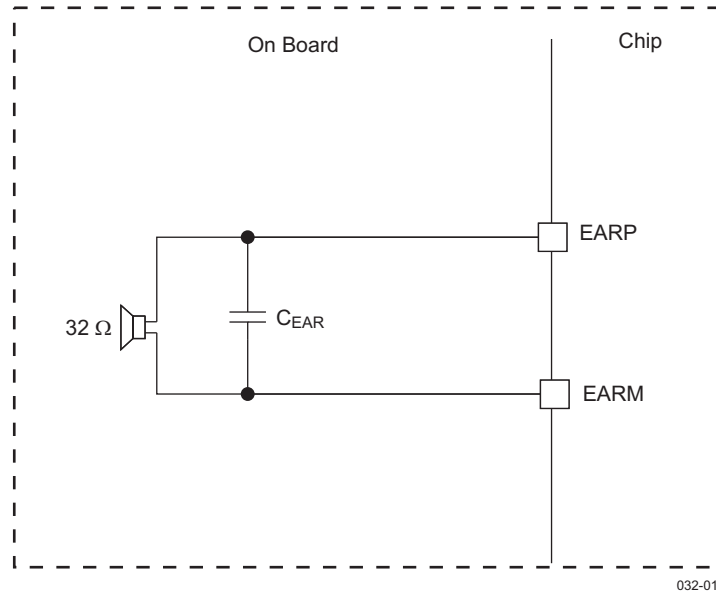
Figure 6-3. Earphone Speaker
