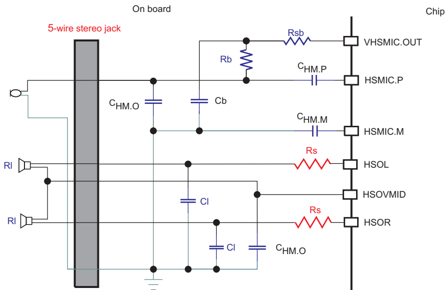
Figure 6-9. Headset 5-Wire Stereo Jack
