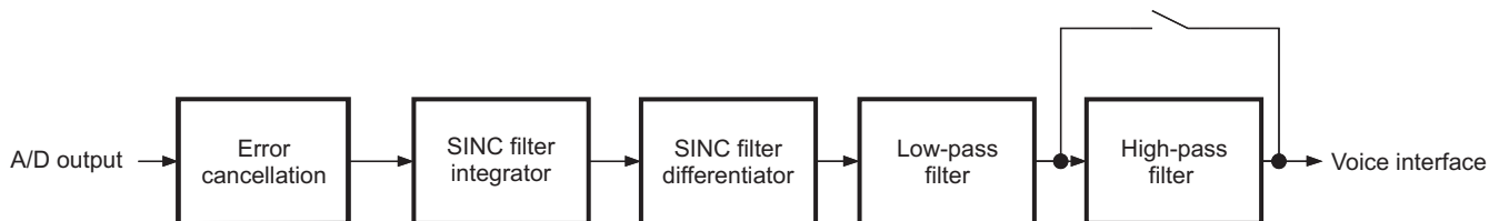
Figure 6-30. Digital Audio Filter Uplink Path Characteristics
